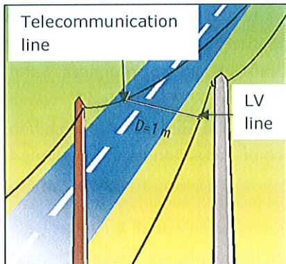
Figure 9: Safety distance between LV overhead line and telephone line
