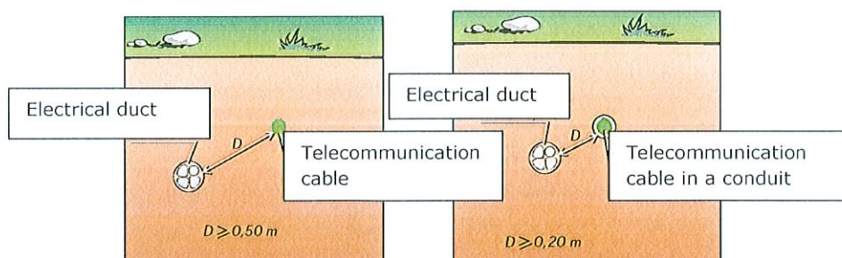
Figure 14: Safety distances between underground conductors and telecommunication cables
